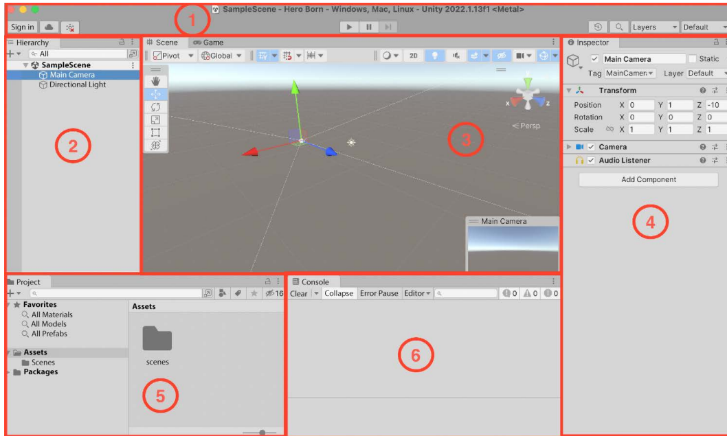
Figure 1.13: Unity interface
