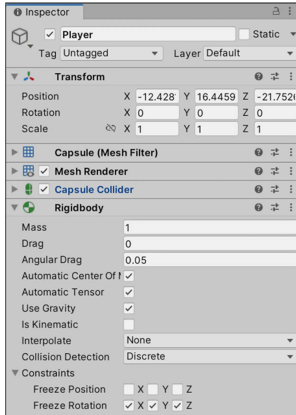
Figure 7.1: Rigidbody component
