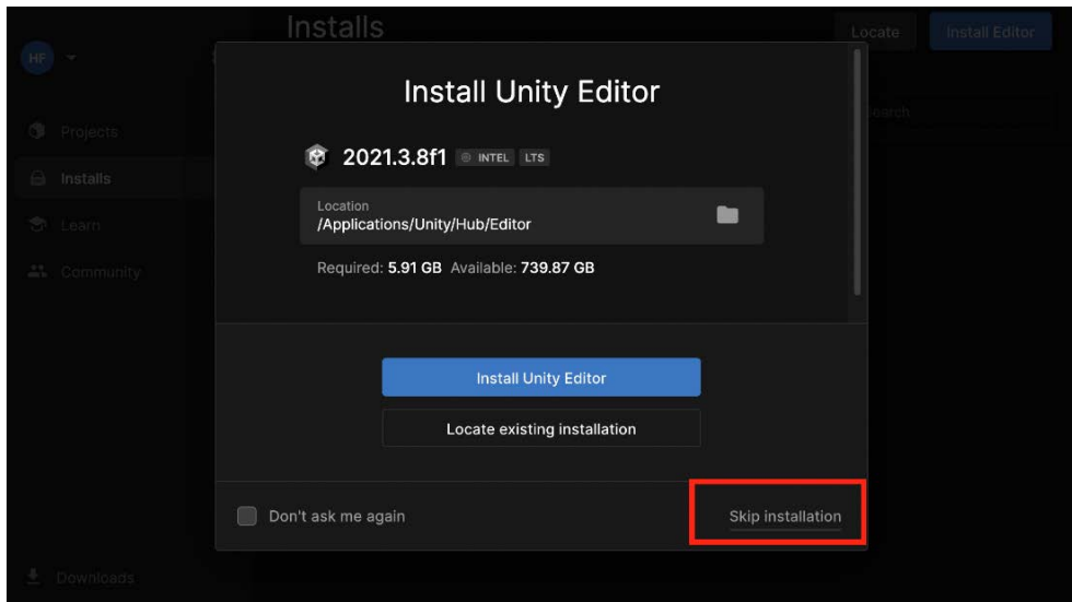
Figure 1.5: Install wizard
