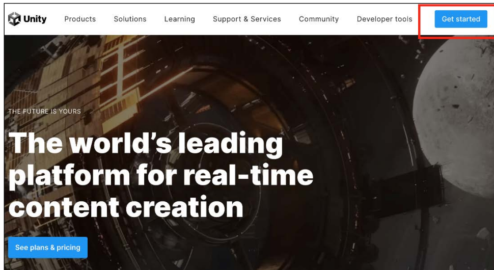
Figure 1.1: Unity homepage
