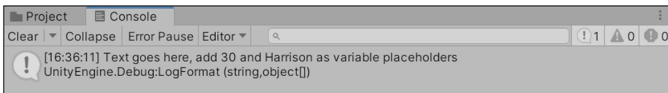
Figure 3.2: Observing Debug.LogFormat
